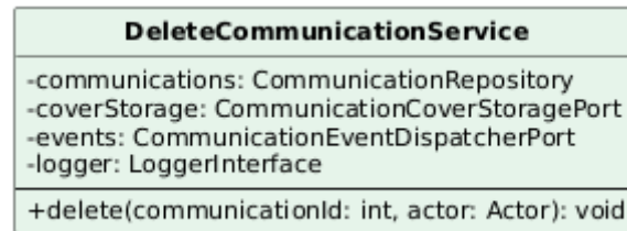
Figura 66: Classe: DeleteCommunicationService
