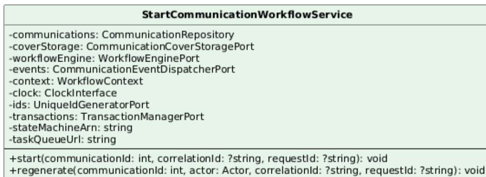
Figura 55: Classe: StartCommunicationWorkflowService
