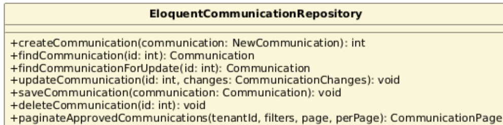
Figura 69: Classe: EloquentCommunicationRepository
